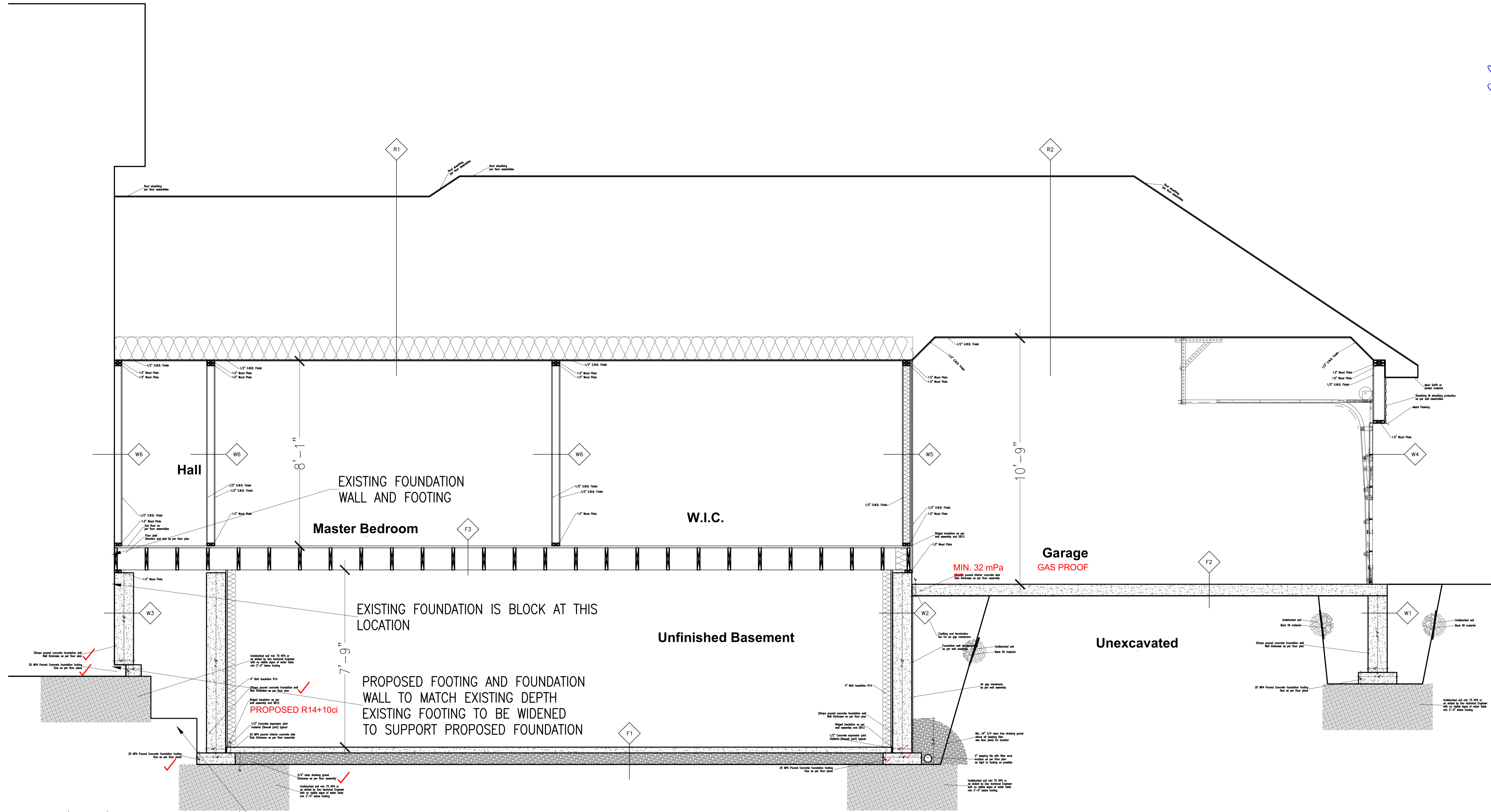
A Section V01 SCALE 1/2" = 1'-0"
